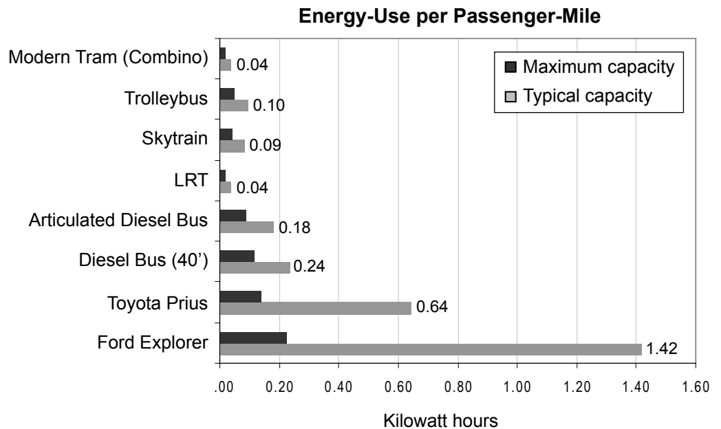
Figure 7. The Toyota Prius is an electric hybrid that provides substantial gains in fuel economy and major reductions in total tailpipe emissions. Reductions in CO2 emissions will vary depending on the source of the electricity that recharges the secondary battery. It has an energy efficiency of 1.5 passenger-miles per kWh.
